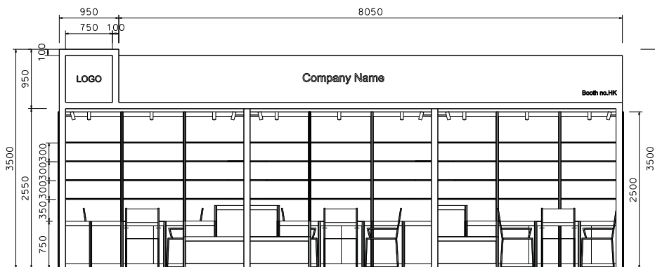
FRONT ELEVATION
