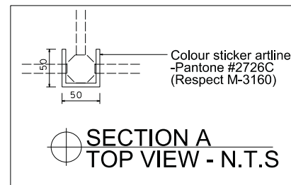
Display podium with colour sticker lamination (Respect M-3160)
