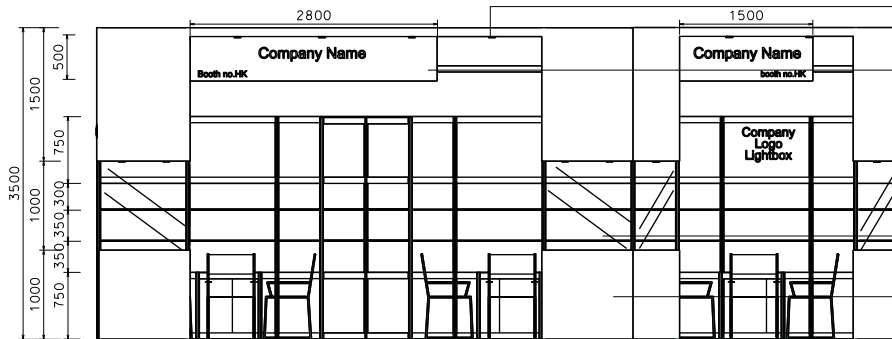
FRONT ELEVATION
