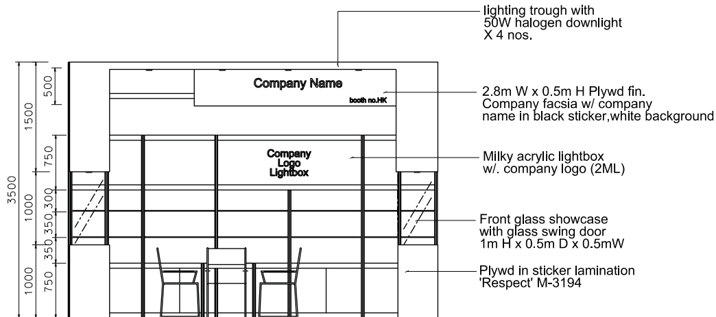
FRONT ELEVATION
