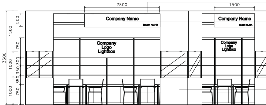
FRONT ELEVATION
